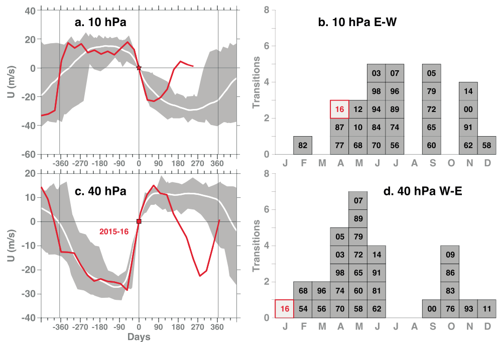
Figure 3. Composite of monthly zonal winds around the QBO transition time from the FUB Singapore-Canton Island-Gan/Malediva Island time series at: (a) 10 hPa and (c) 40 hPa. As noted in the text, the time of the transition is calculated from the QBO time series (27 events), and each event is then shifted to this “day 0” (i.e., phase rectified). Transition dates are noted in Figure 1 as red squares for 40 hPa E-W and red stars for 10 hPa W-E. The white line shows the average of the 27 events, while the grey shading shows the minimum to maximum range of all of the QBOs (excluding the 2015–2016 event). The 2015–2016 event is plotted in red. The vertical black lines show \pm 1 year. Also shown in the right panels are the months when: (b) the easterly to westerly transition occurs at 10 hPa and (d) the westerly to easterly transition occurs at 40 hPa. In Figures 3b and 3d the boxes are labeled by year with 2016 highlighted in red.
