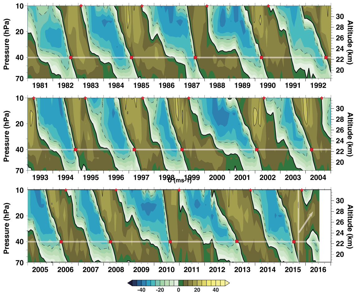
Figure 1. Monthly mean zonal wind ( \text{m s}^{-1} ) derived from Singapore radiosondes ( 1^\circ\text{N} , 104^\circ\text{E} ) between 70 and 10 hPa for 1981 through July 2016. The color scale is on the bottom with 5 \text{ m s}^{-1} color increments. Easterlies are shown in cyan blue, while westerlies are in green brown. Contours are every 20 \text{ m s}^{-1} , with easterlies dashed and westerlies solid, and a thick black zero wind. The red squares show the dates of the 40 hPa easterly-to-westerly transition, while the red stars show the 10 hPa dates of the westerly to easterly transition.
