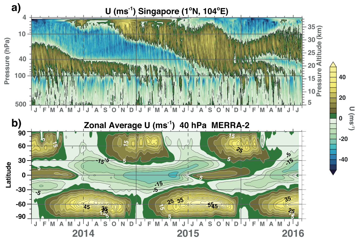
Figure 2. Daily zonal winds (January 2014 through July 2016) for (a) altitude-time plot of Singapore radiosondes and (b) latitude-time plot of MERRA-2 zonal mean zonal winds at 40 hPa. Easterlies are shown in cyan blue, while westerlies are in green brown.
