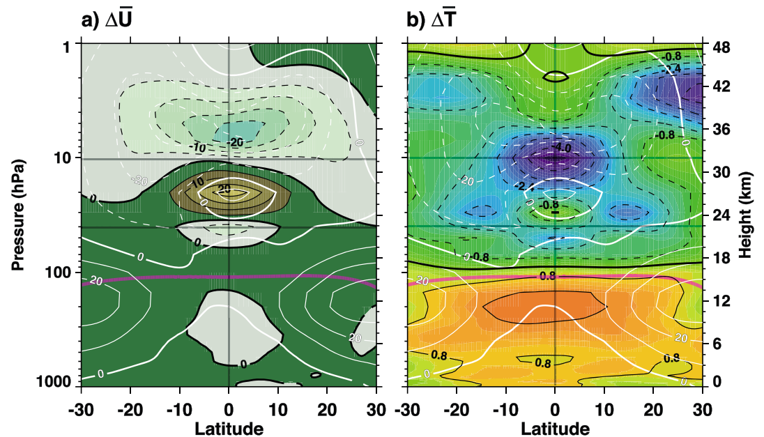
Figure 4. The January–May 2016 deviations from the January–May 1980–2015 average of (a) zonal mean zonal wind and (b) temperature, as computed from MERRA-2. Both panels have the January–May 2016 averaged zonal mean zonal winds (white lines) and tropopause (thick magenta line). Units are \text{m s}^{-1} and K.
