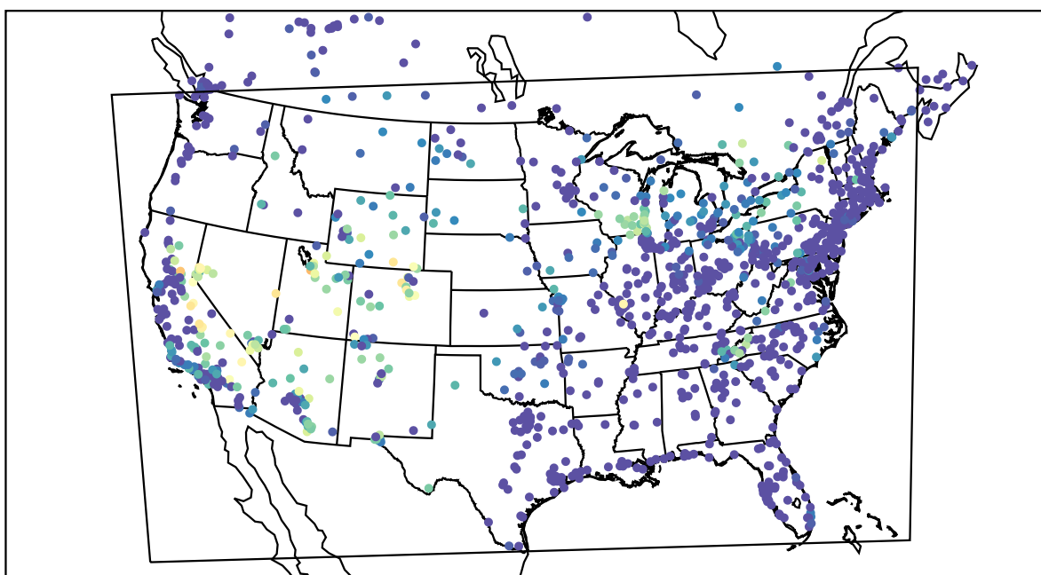
AirNOW (2019-07-19_11:00:00)
