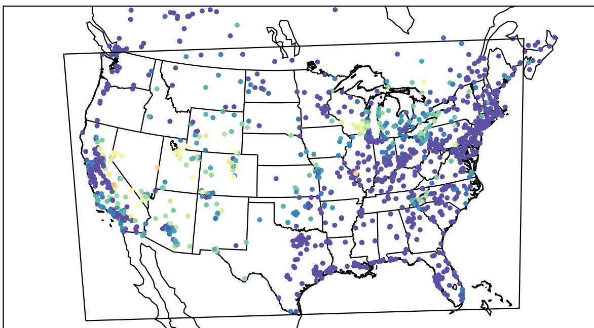
AirNOW (2019-07-19_09:00:00)
