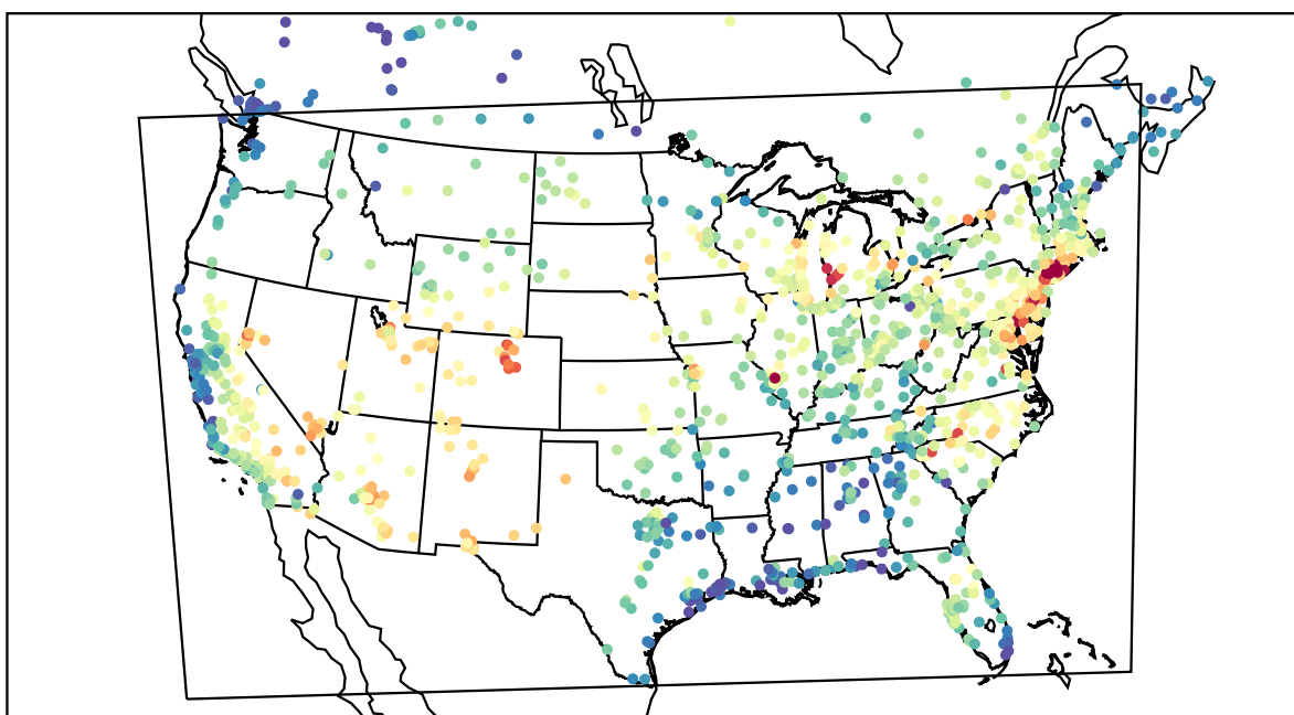
AirNOW (2019-07-19_19:00:00)
