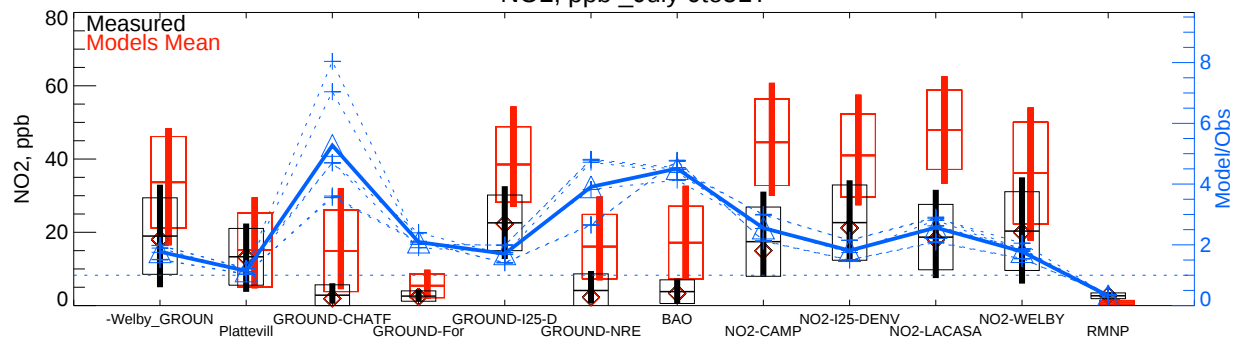
NO2, ppb _July 8to12LT
