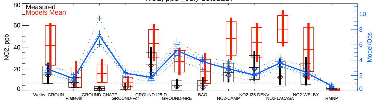
NO2, ppb _July 18to22LT
