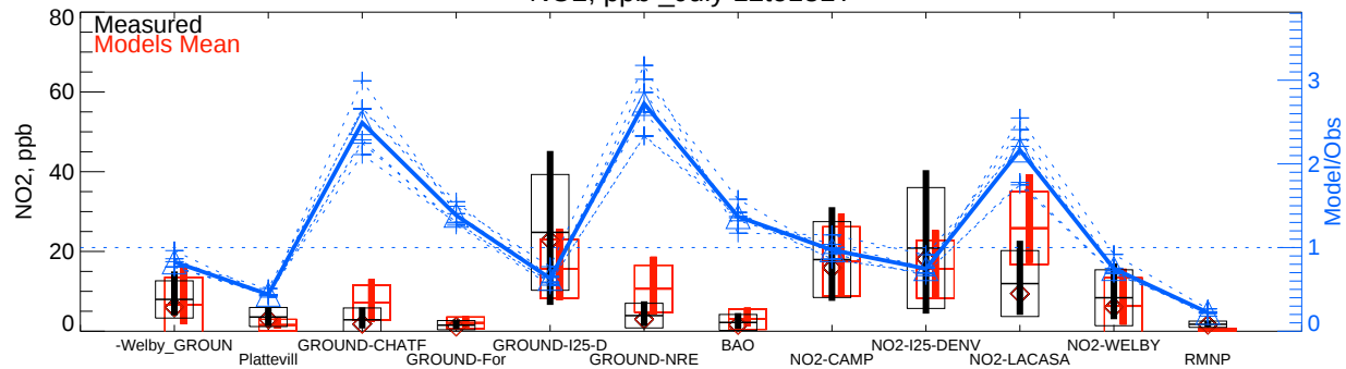
NO2, ppb _July 18to22LT
