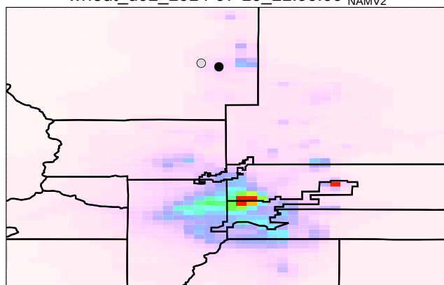
NOx Surface
