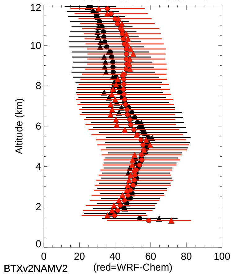
RH Observations Platteville
