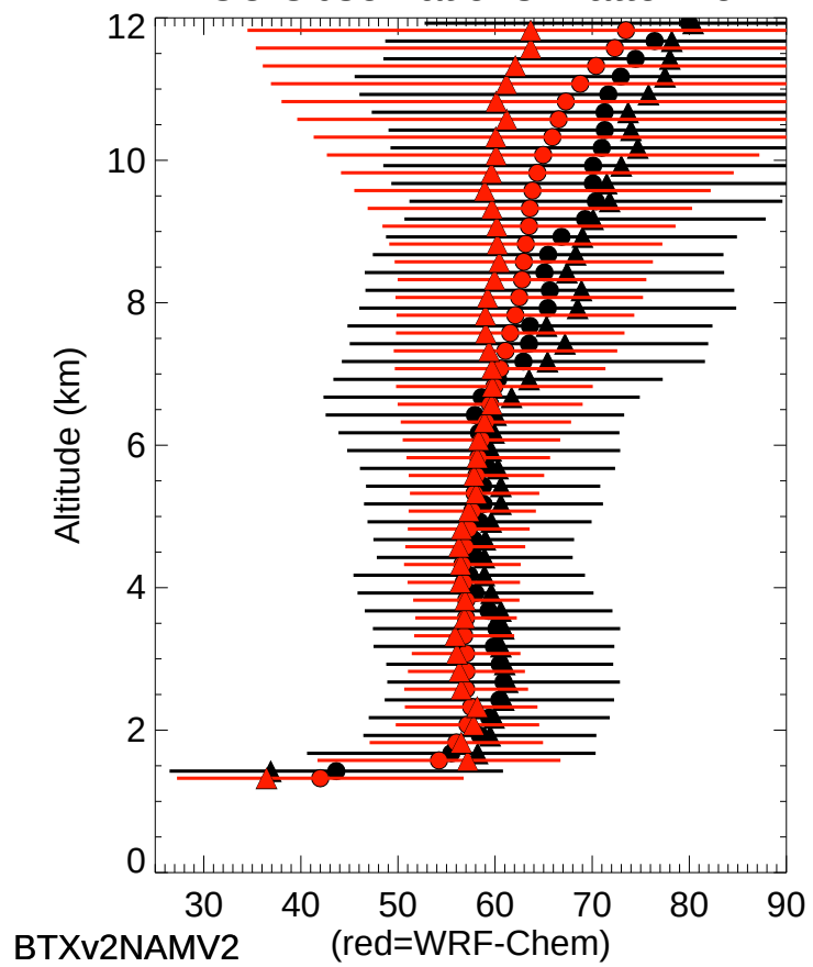
O3 Observations Platteville
