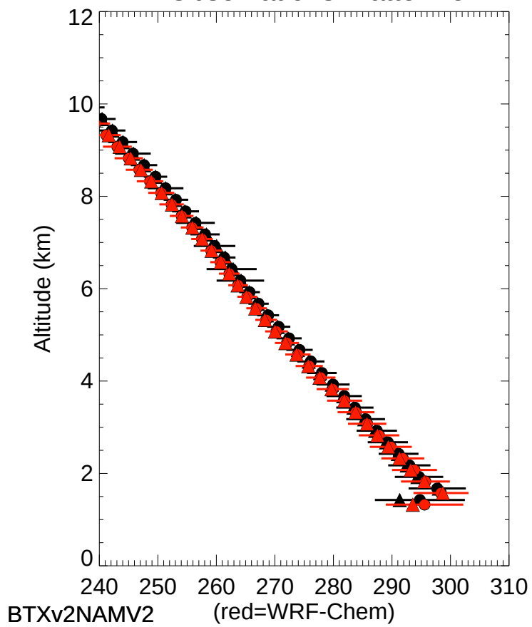
T Observations Platteville
