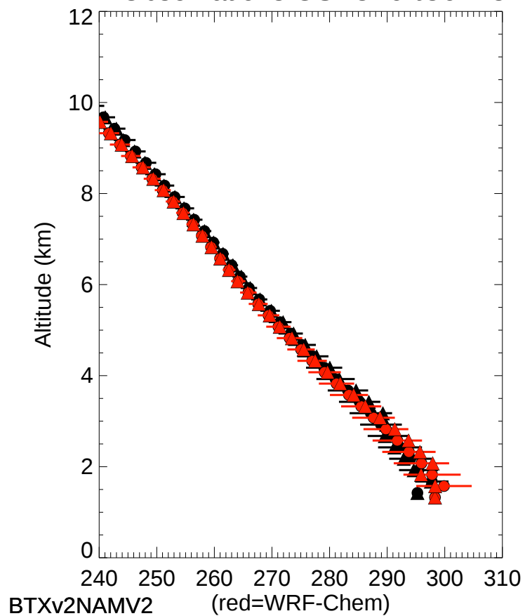
T Observations GSFCFortCollins
