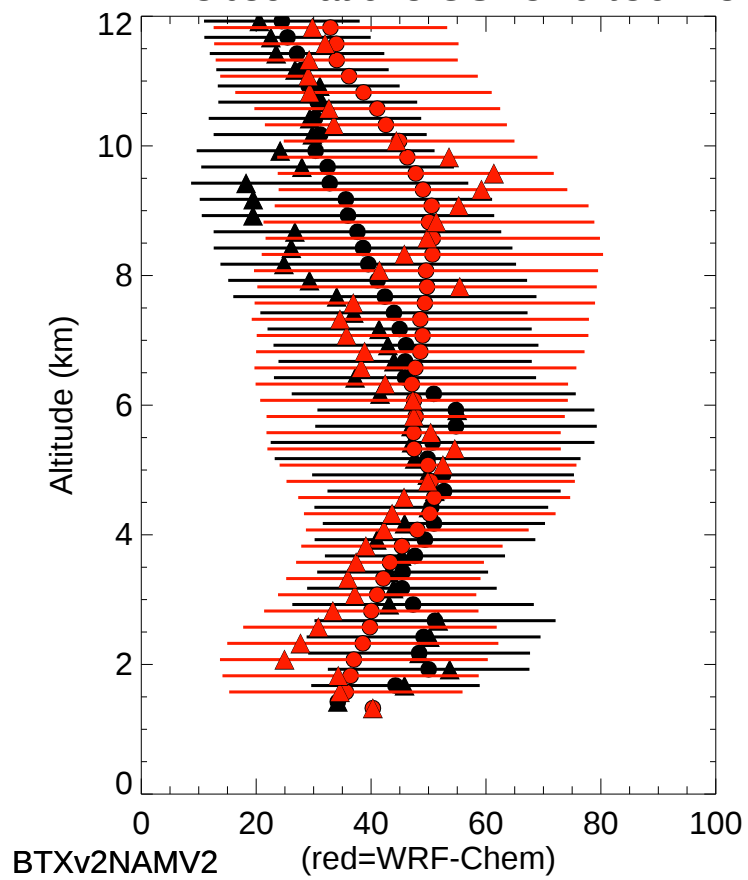
RH Observations GSFCFortCollins
