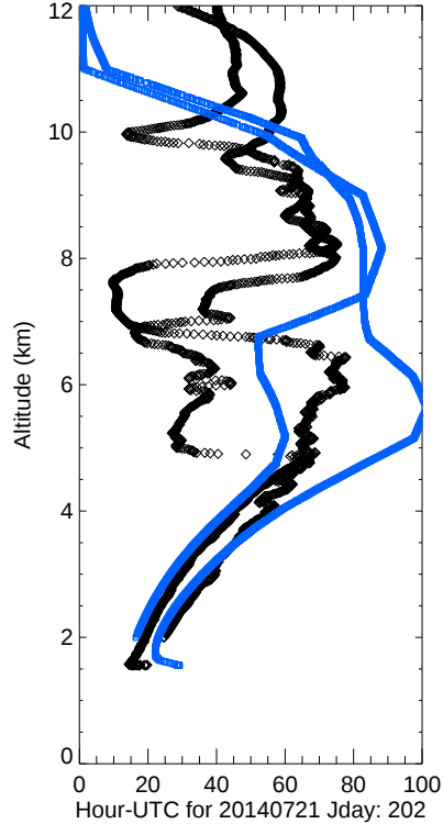
RH Observations GSFCFortCollins
