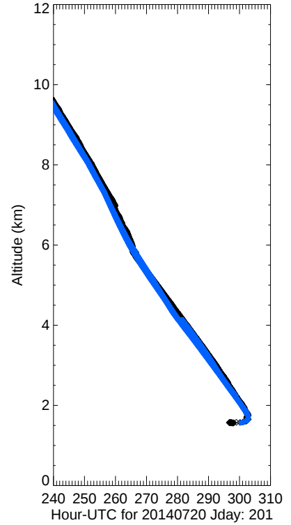
T Observations GSFCFortCollins
