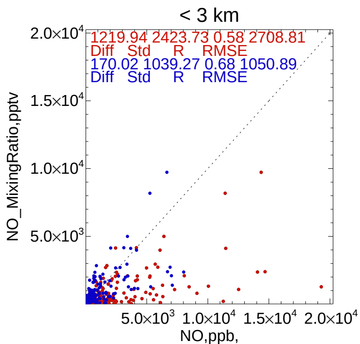
Model-Obs(%) NO,ppb, < 3 km
