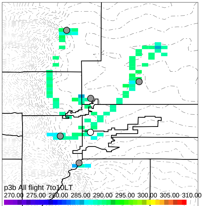
TEMPERATURE,K < 3 km
