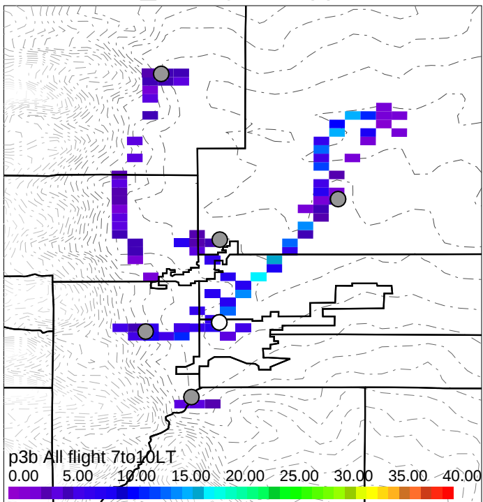
Ammonia_MixingRatio,ppbv < 3 km
