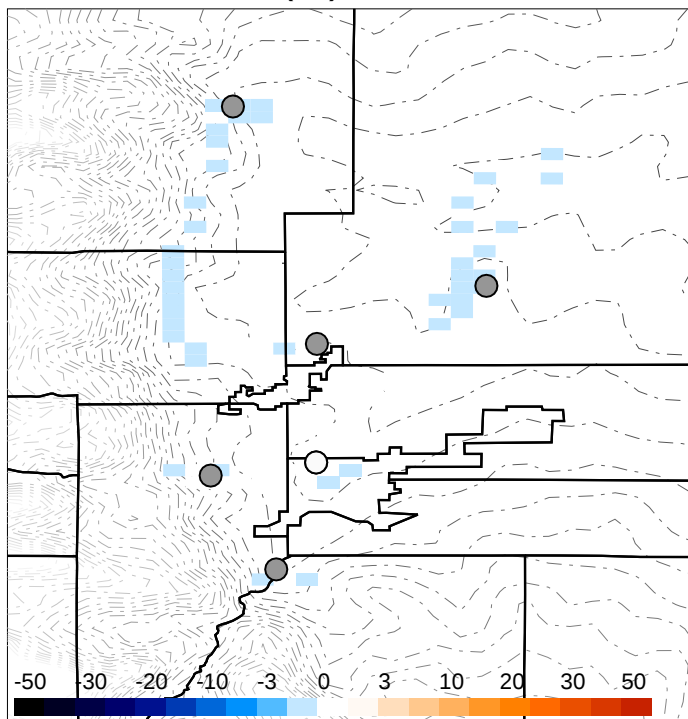
Model-Obs(%) Tair,K, < 3 km
