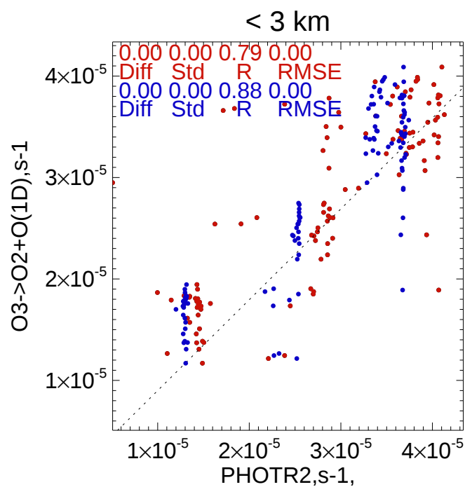
Model-Obs(%) PHOTR2,s-1, < 3 km
