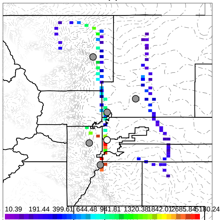
Model NO2,ppb, < 3 km
