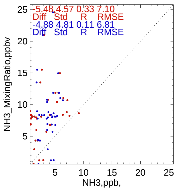
< 3 km
