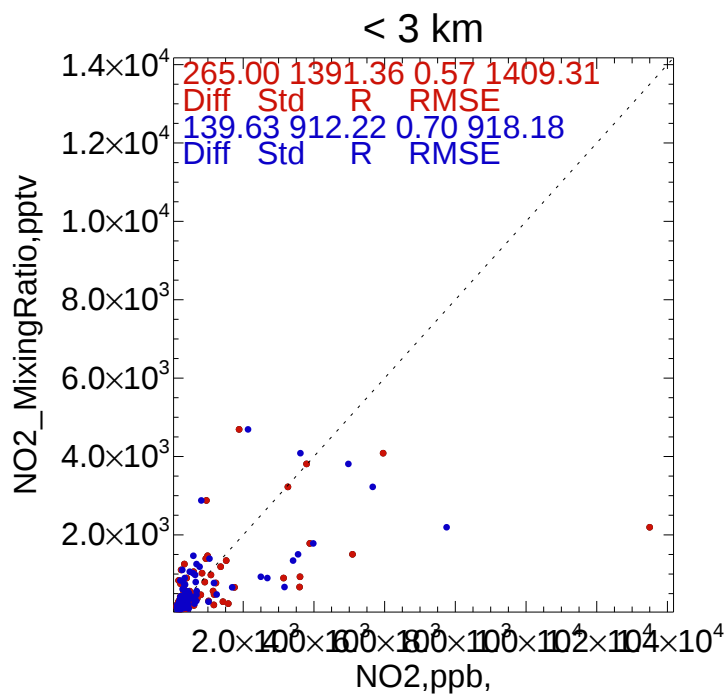
Model-Obs(%) NO2,ppb, < 3 km
