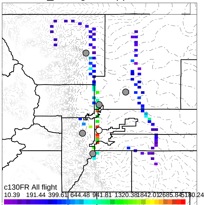
NO2_MixingRatio,pptv < 3 km
