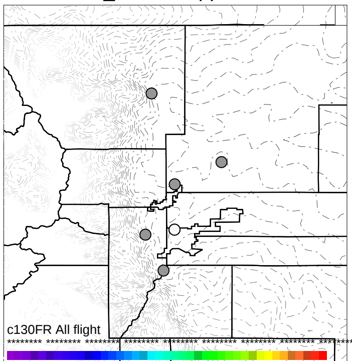
HNO 3 _GTCIMS,pptv > 3 km
