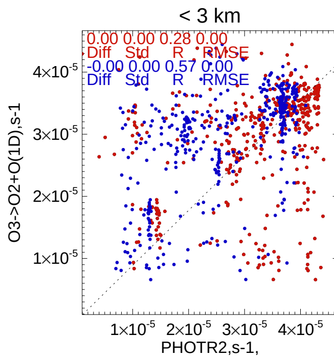
Model-Obs(%) PHOTR2,s-1, < 3 km
