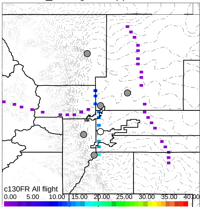
NH3_MixingRatio,ppbv > 3 km
