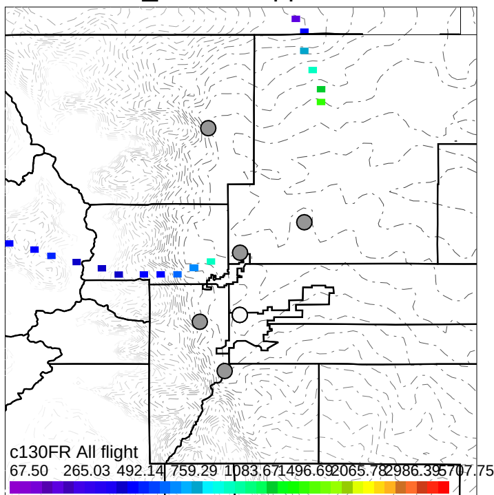
HNO 3 _GTCIMS, pptv > 3 km
