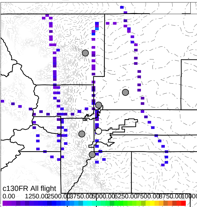
C2H6_CAMS, pptv > 3 km
