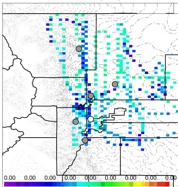
Model PHOTR2,s-1, < 3 km
