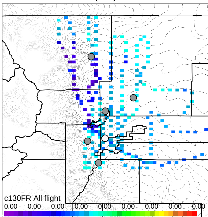
Model-Obs(%) PHOTR2,s-1, < 3 km
