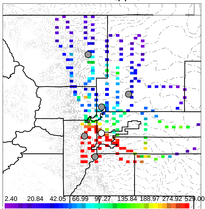
Model TOLUENE, ppb, < 3 km
