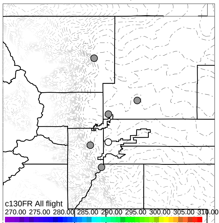
Model-Obs(%) Tair,K, > 3 km
