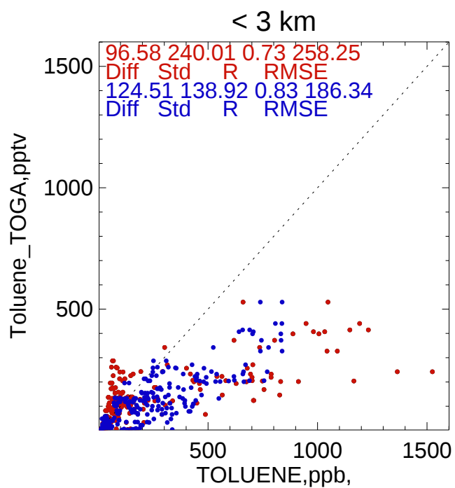
Model-Obs(%) TOLUENE, ppb, < 3 km
