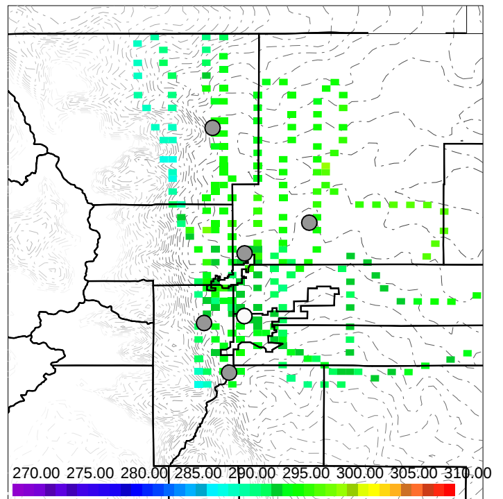
Model Tair,K, < 3 km
