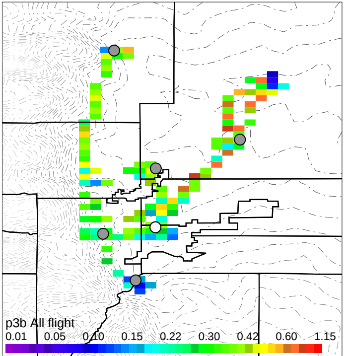
MEK-butanal_MixingRatio,ppbv < 3 km
