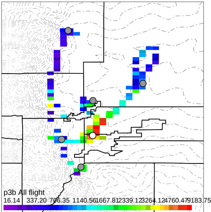
Model-Obs(%) NO2,ppb, < 3 km
