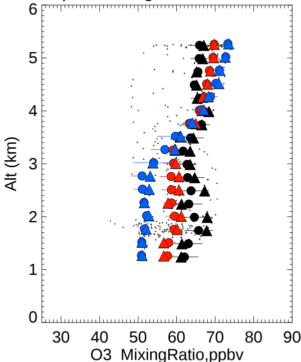
p3b All flight FortCollins
