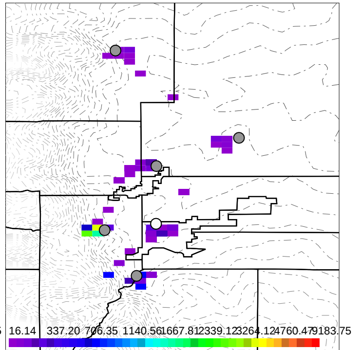
Model NO2,ppb, > 3 km
