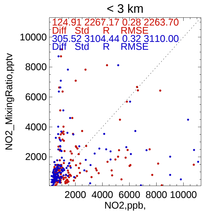
Model-Obs(%) NO2,ppb, < 3 km
