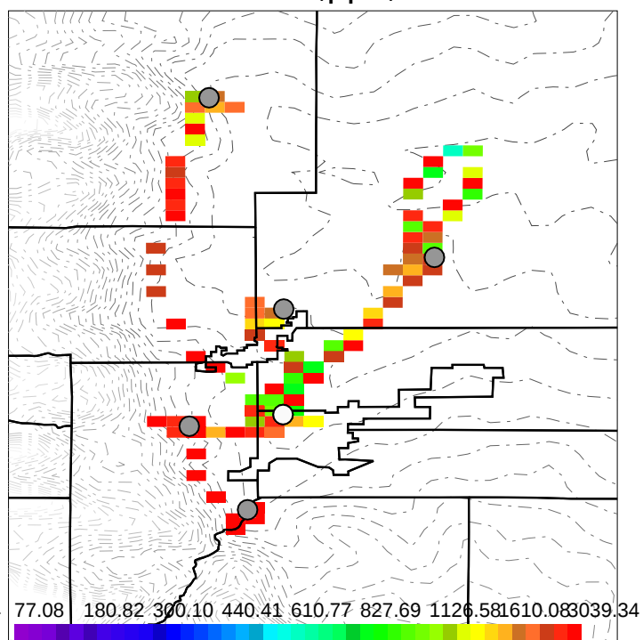
Model HNO 3 ,ppb, < 3 km
