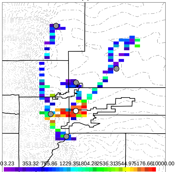
Model NO,ppb, < 3 km
