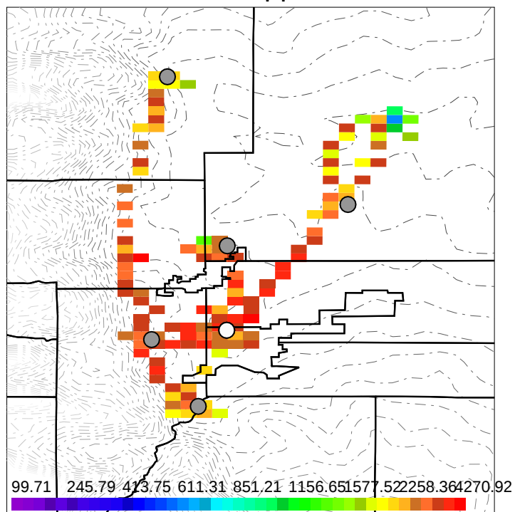
Model HCHO,ppb, &lt; 3 km
