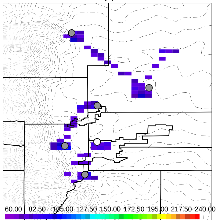
Model CO,ppb, > 3 km
