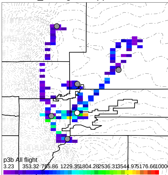
NO_MixingRatio,pptv < 3 km
