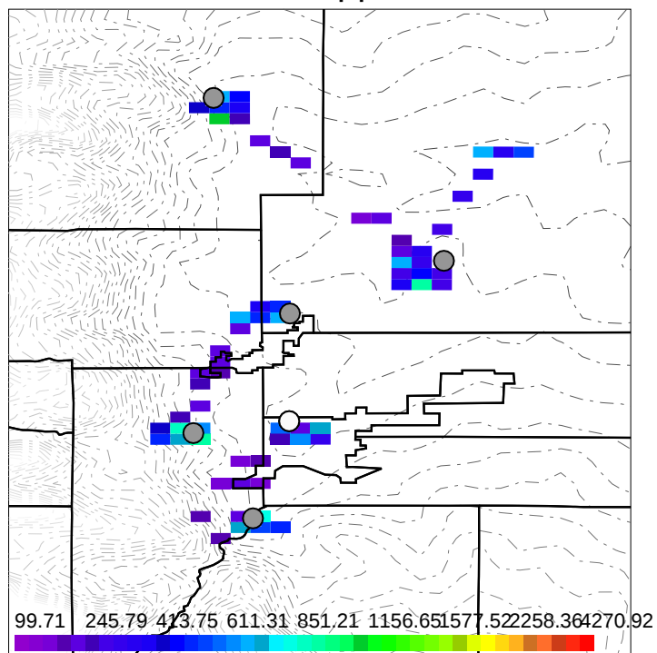
Model HCHO,ppb, &gt; 3 km
