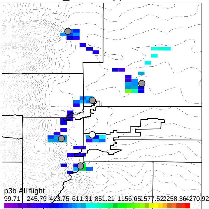
Model-Obs(%) HCHO,ppb, &gt; 3 km
