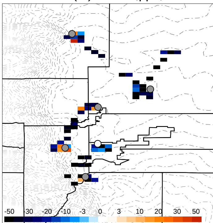
Model-Obs(%) HCHO,ppb, &gt; 3 km
