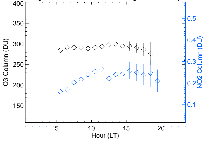
P28_ground-Fort-Collins Average Diurnal Cycle
