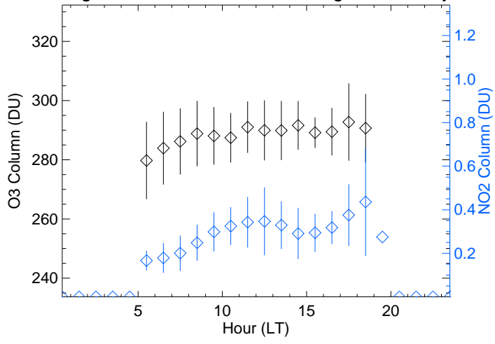
P39_ground-NREL-Golden Average Diurnal Cycle
