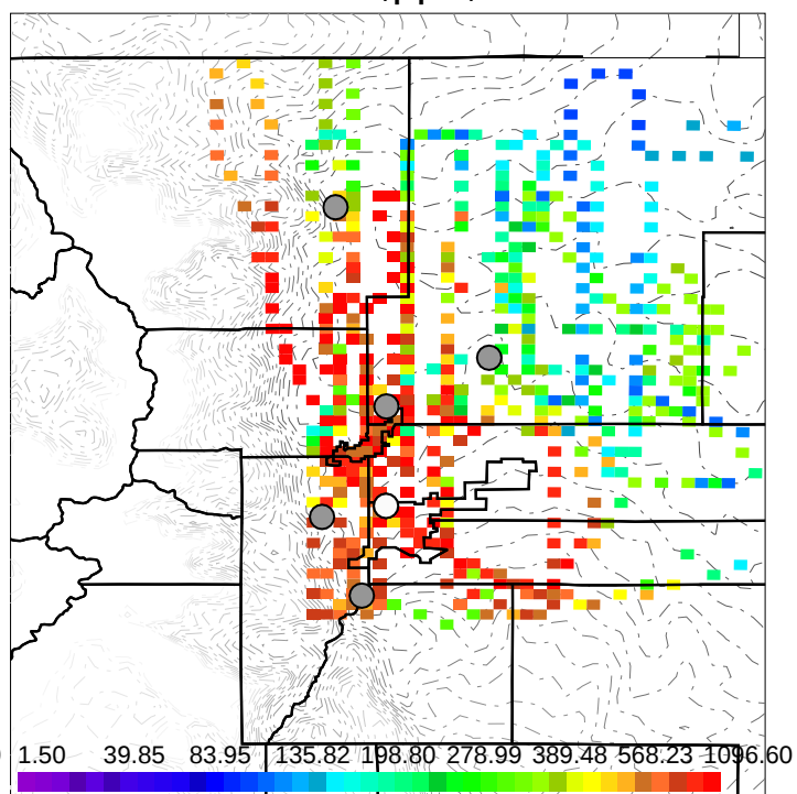
Model MEK, ppb, < 3 km
