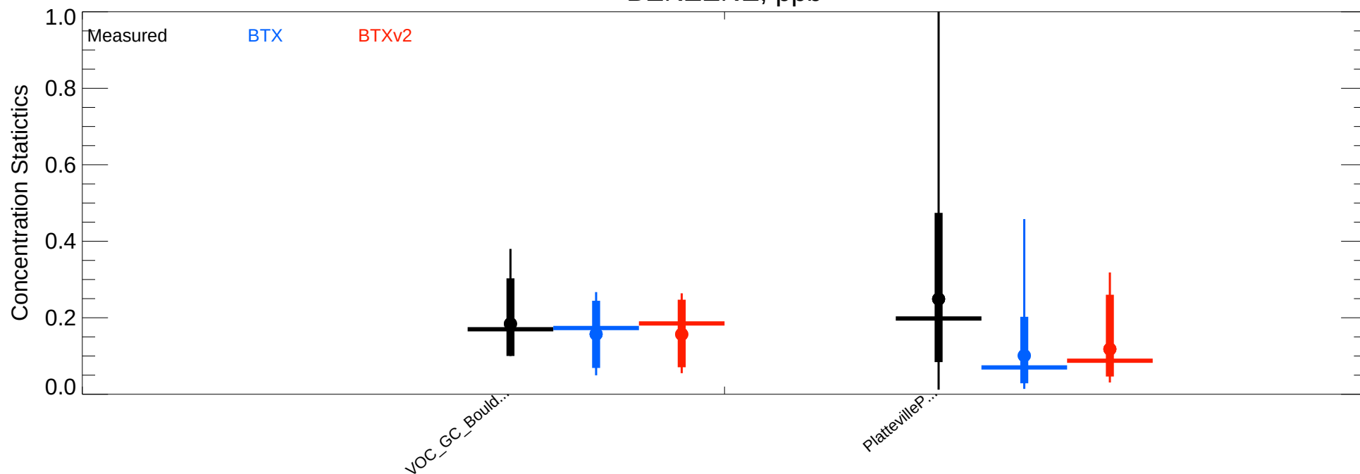
BENZENE, ppb
