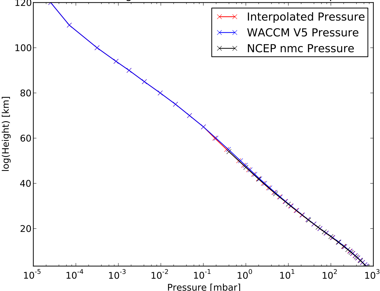
Pressure vs Height for Date:2013-01-11, K = 3, nskips = 1
