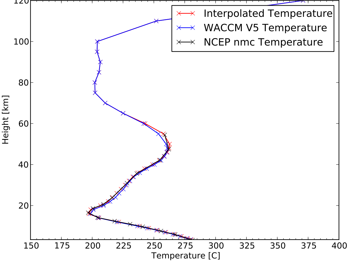
Temperature vs Height for Date:2014-10-25, K = 2, nskips = 1
