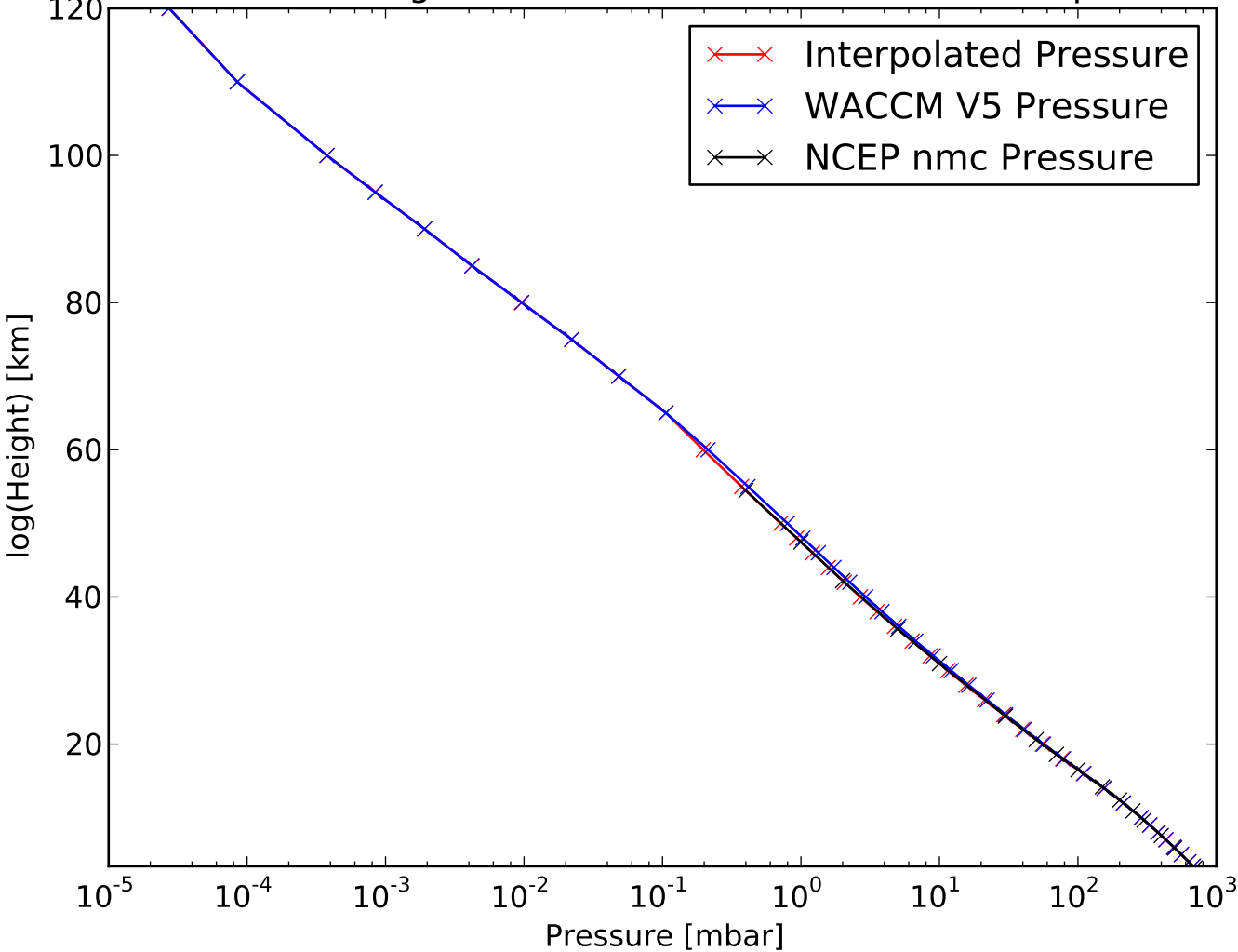
Pressure vs Height for Date:2014-10-25, K = 3, nskips = 1
