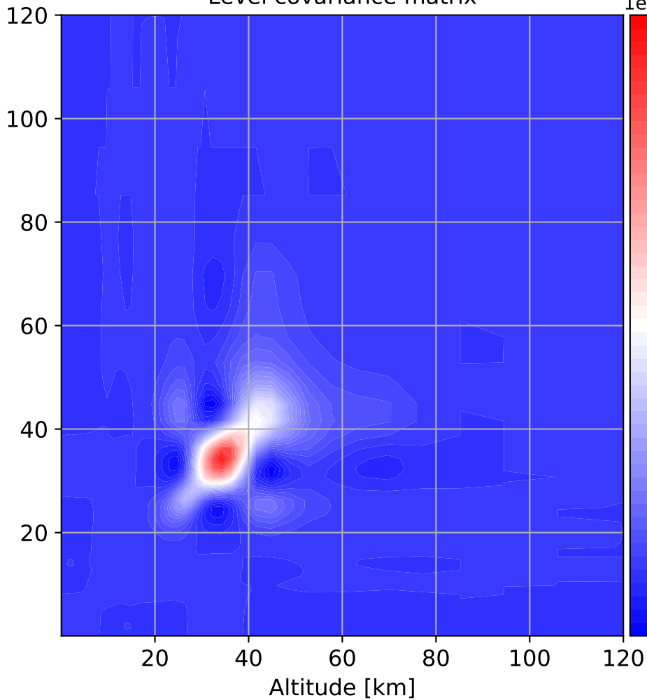
Level covariance matrix
