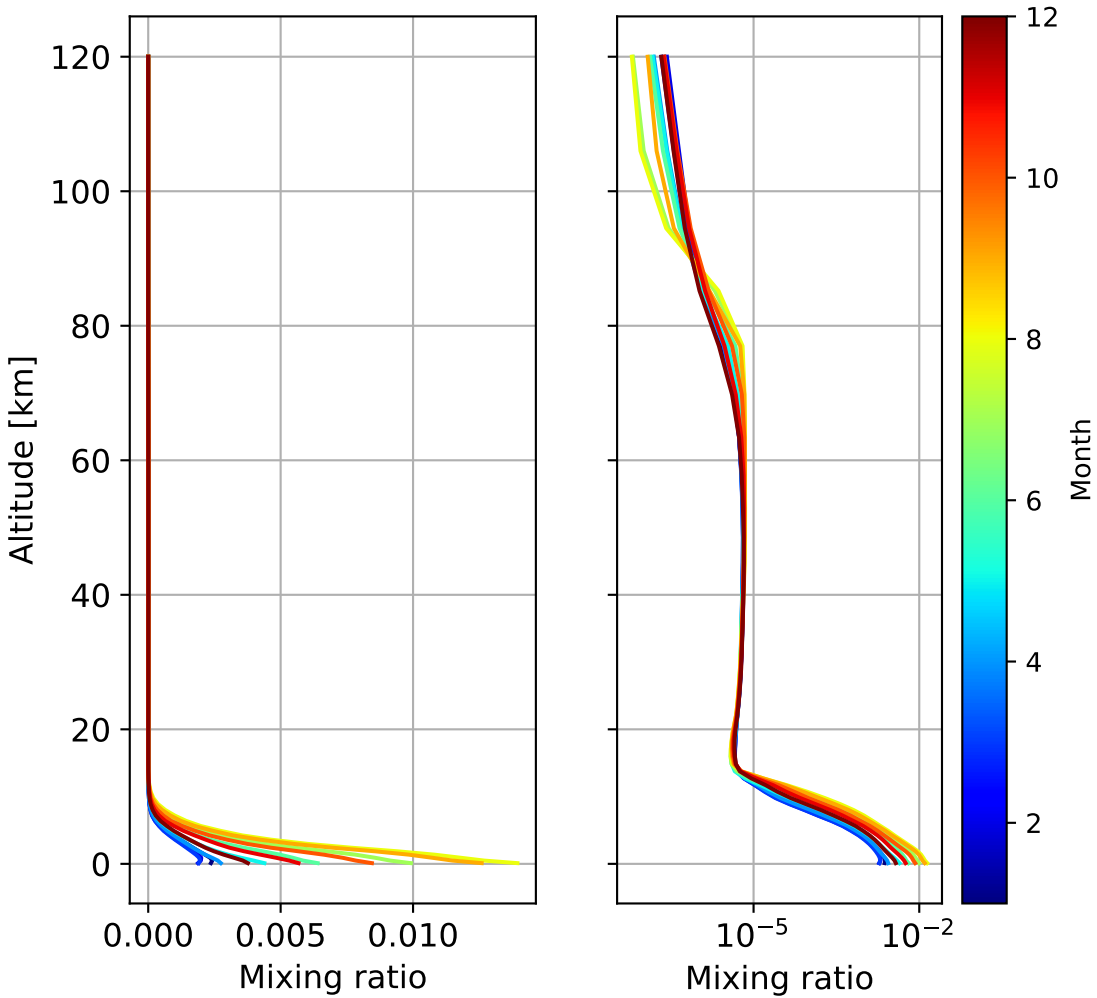
Monthly mean WACCM profile (interpolated to station grid) Tomsk, 56.475N, 85.046E, 0.106kmasl
