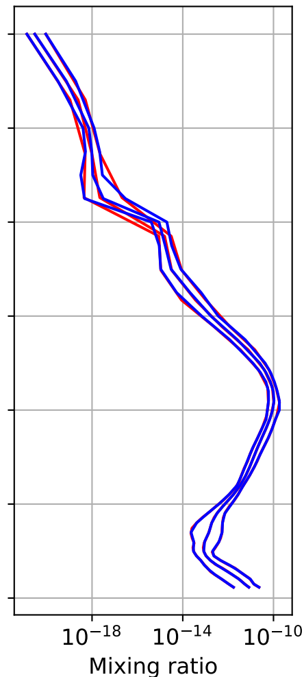
Min, Max, Mean of 732 profiles Table_Mtn, 34.4N, 242.3E, 2.3kmasl
