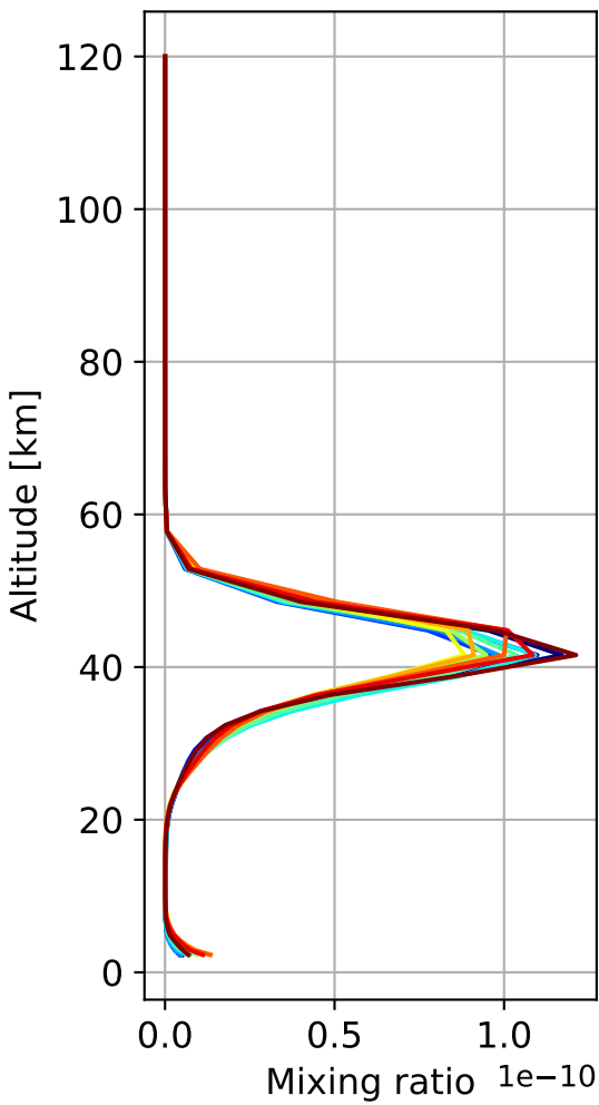
Monthly mean WACCM profile (interpolated to station grid) Table_Mtn, 34.4N, 242.3E, 2.3kmasl
