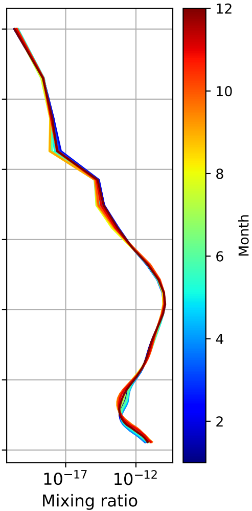
Monthly mean WACCM profile (interpolated to station grid) Table_Mtn, 34.4N, 242.3E, 2.3kmasl
