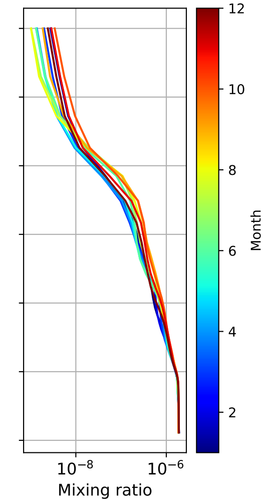
Monthly mean WACCM profile (interpolated to station grid) Table_Mtn, 34.4N, 242.3E, 2.3kmasl
