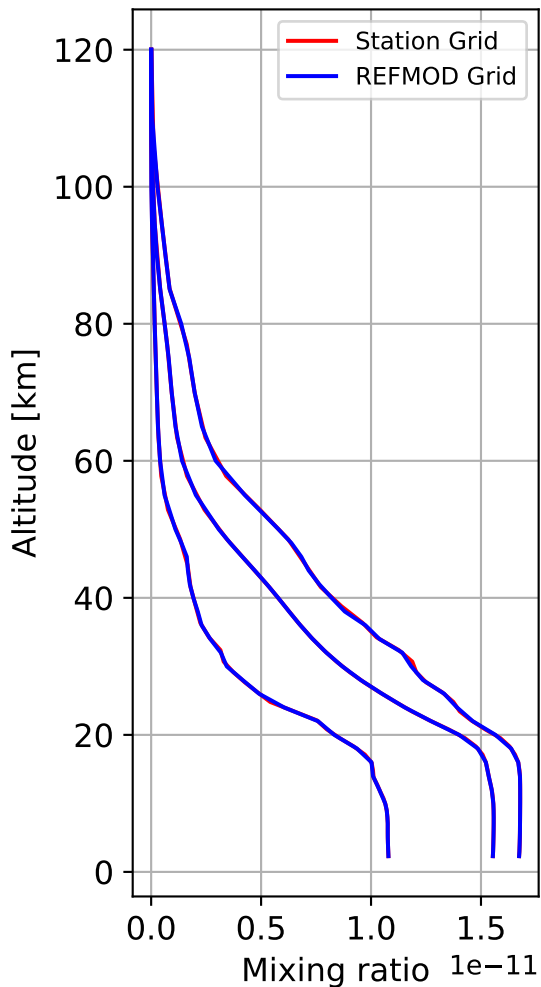
Min, Max, Mean of 732 profiles Table_Mtn, 34.4N, 242.3E, 2.3kmasl
