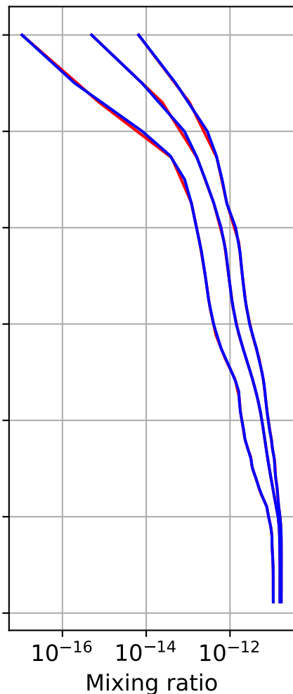
Min, Max, Mean of 732 profiles Table_Mtn, 34.4N, 242.3E, 2.3kmasl
