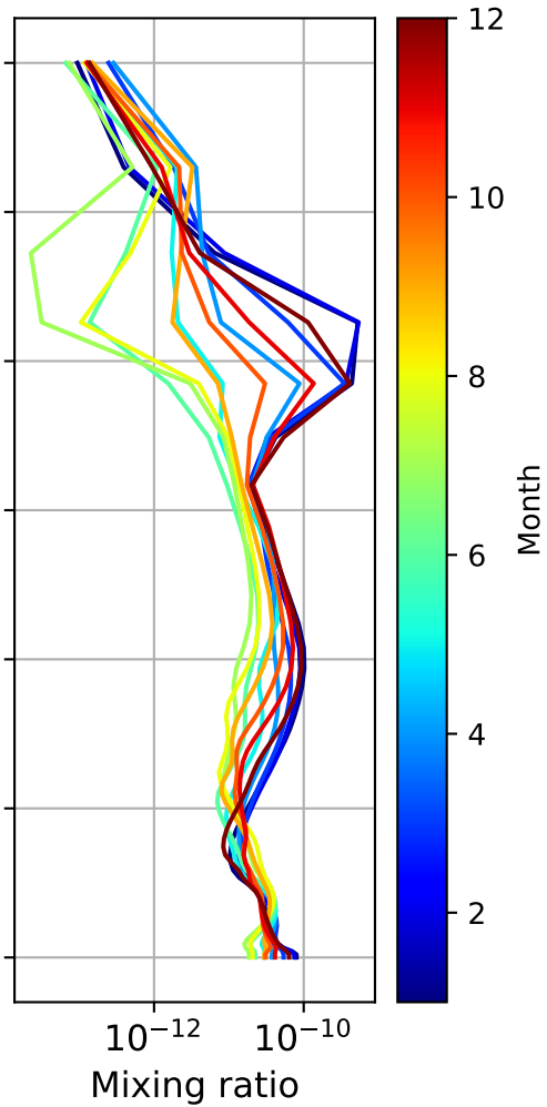
Monthly mean WACCM profile (interpolated to station grid) Syowa_Station, -69.0N, 39.59E, 0.01kmasl
