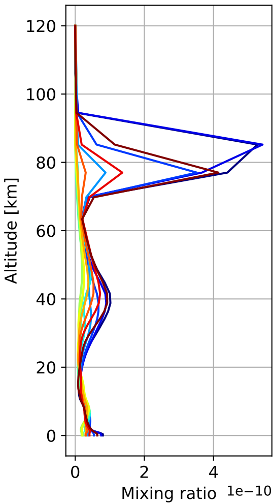
Monthly mean WACCM profile (interpolated to station grid) Syowa_Station, -69.0N, 39.59E, 0.01kmasl
