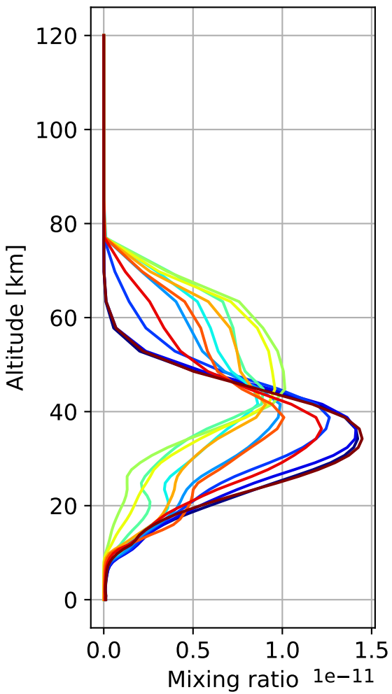
Monthly mean WACCM profile (interpolated to station grid) Syowa_Station, -69.0N, 39.59E, 0.01kmasl
