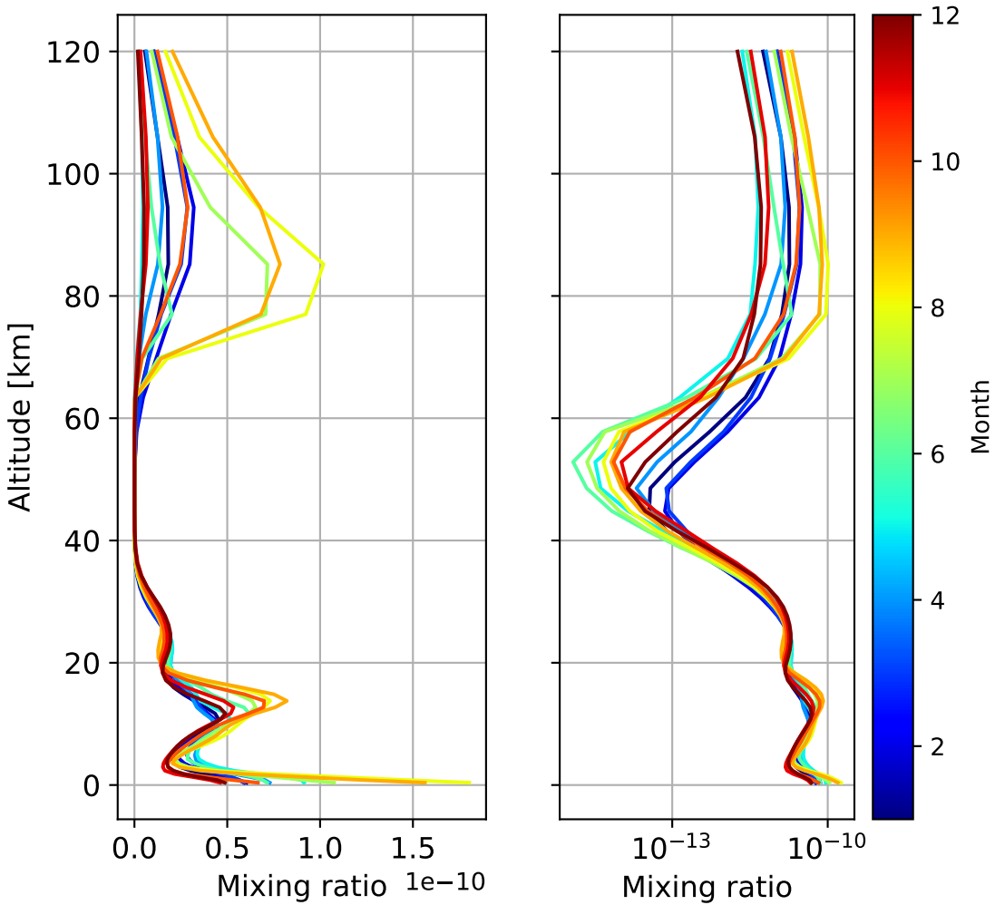
Monthly mean WACCM profile (interpolated to station grid) Rikubetsu, 43.46N, 143.77E, 0.38kmasl
