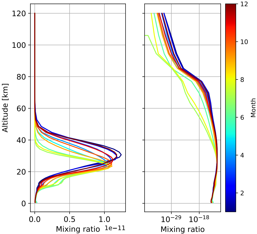
Monthly mean WACCM profile (interpolated to station grid) Poker_Flat, 65.12N, 212.57E, 0.61kmasl
