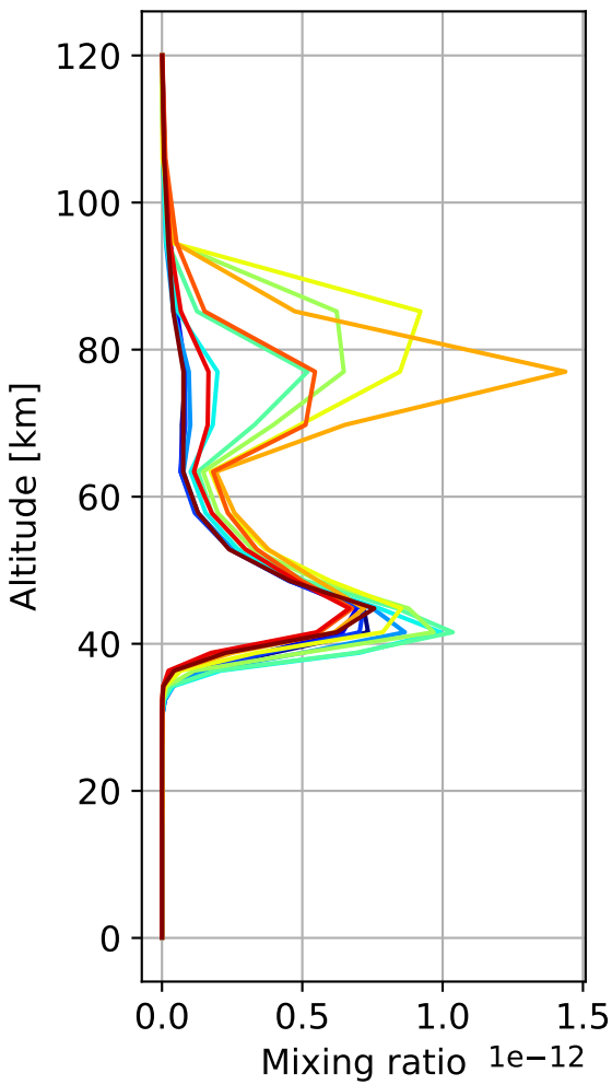
Monthly mean WACCM profile (interpolated to station grid) Paris, 48.97N, 2.37E, 0.06kmasl
