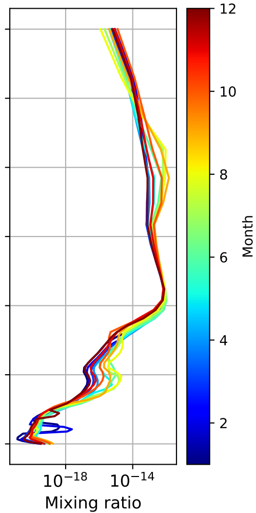
Monthly mean WACCM profile (interpolated to station grid) Paris, 48.97N, 2.37E, 0.06kmasl
