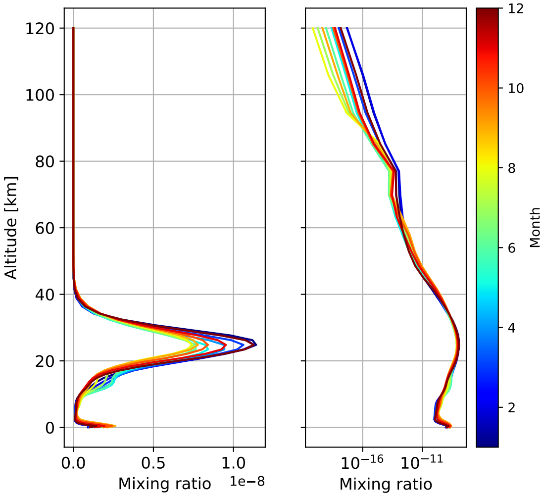
Monthly mean WACCM profile (interpolated to station grid) Paris, 48.97N, 2.37E, 0.06kmasl
