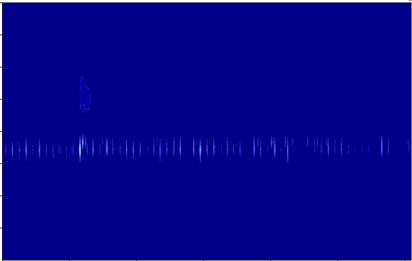
Time Series of vertical profiles (site altitude - 40 km)
