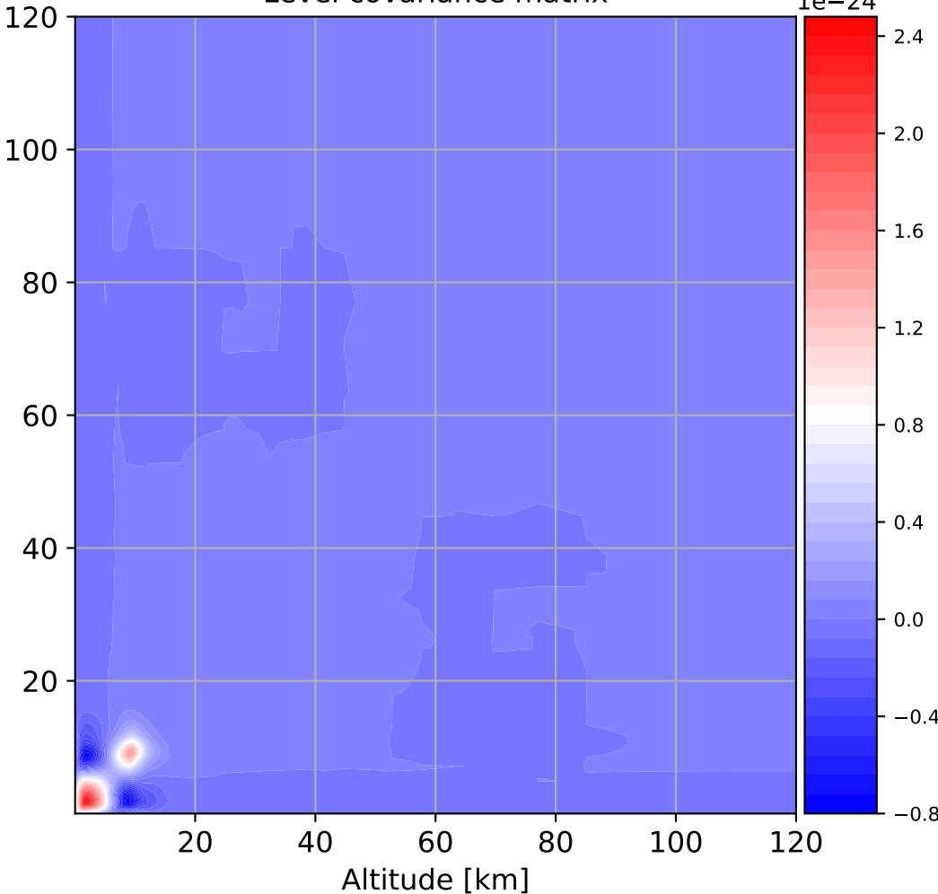
Level covariance matrix
