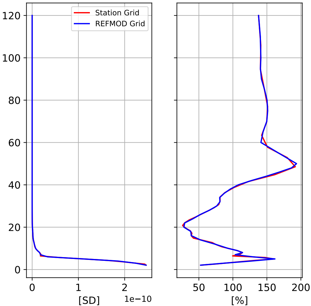
Std. Deviation
