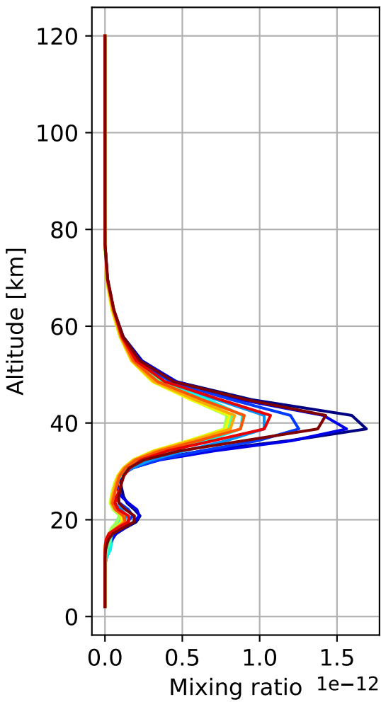
Monthly mean WACCM profile (interpolated to station grid) Kitt_Peak, 31.96N, 248.41E, 2.06kmasl
