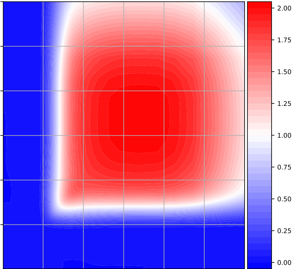
Level covariance matrix
