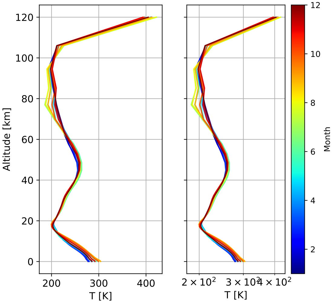
Monthly mean WACCM profile (interpolated to station grid) Hefei, 31.9N, 117.17E, 0.04kmasl
