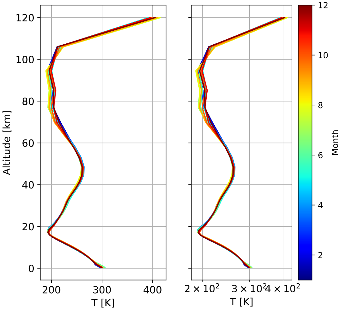
Monthly mean WACCM profile (interpolated to station grid) Gadanki, 13.45N, 79.18E, 0.36kmasl
