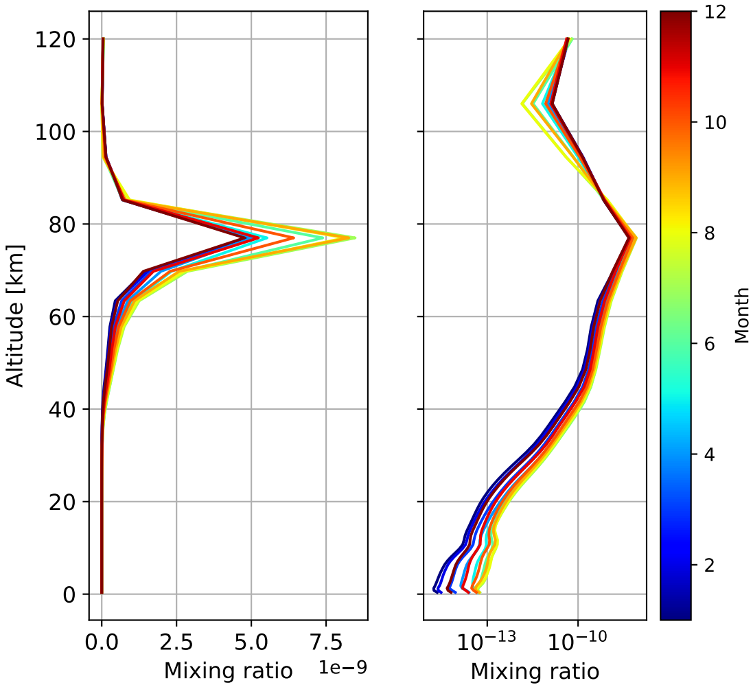
Monthly mean WACCM profile (interpolated to station grid) Fort_McMurray, 56.65N, 248.78E, 0.369kmasl
