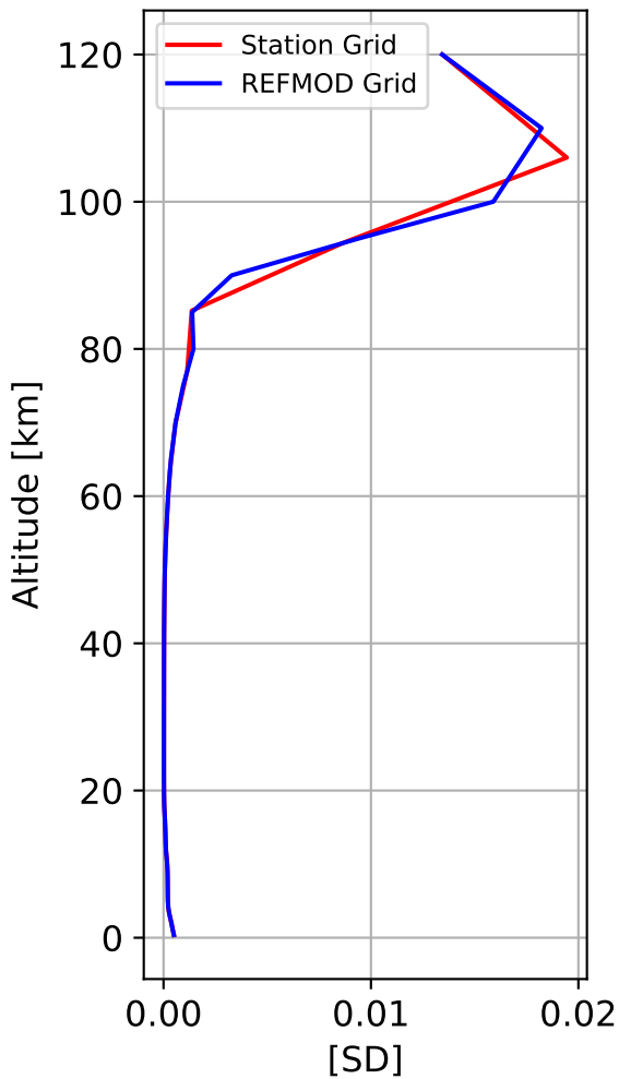
Std. Deviation
