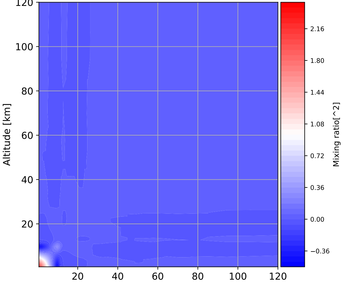
Level covariance matrix
