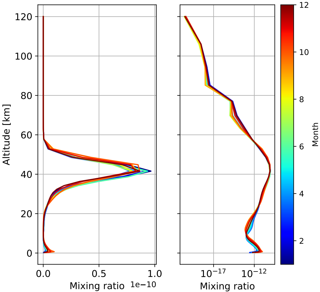
Monthly mean WACCM profile (interpolated to station grid) Egbert, 44.217N, 280.233E, 0.251kmasl
