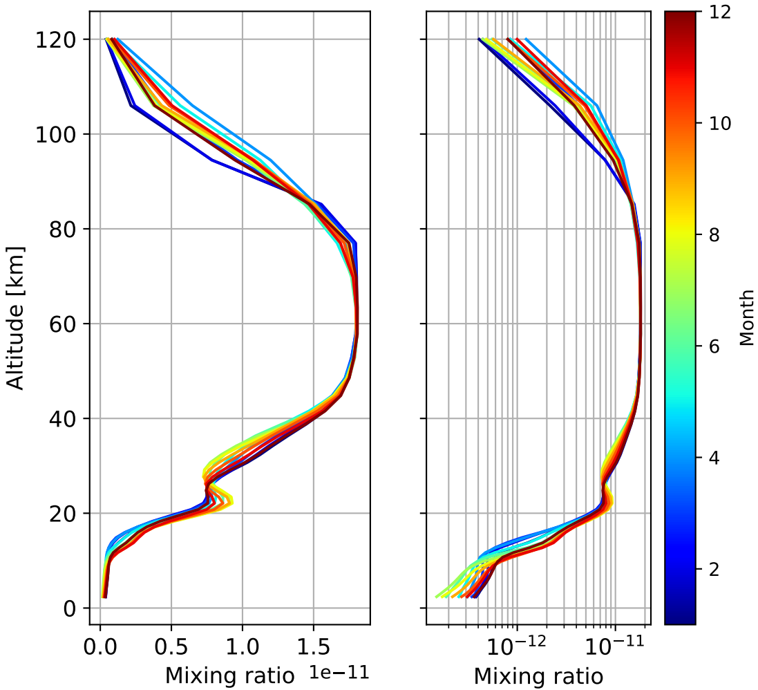
Monthly mean WACCM profile (interpolated to station grid) CTIO, -30.169N, 289.194E, 2.379kmasl
