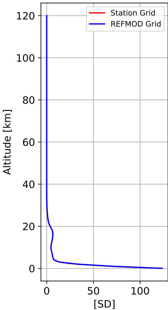
Std. Deviation
