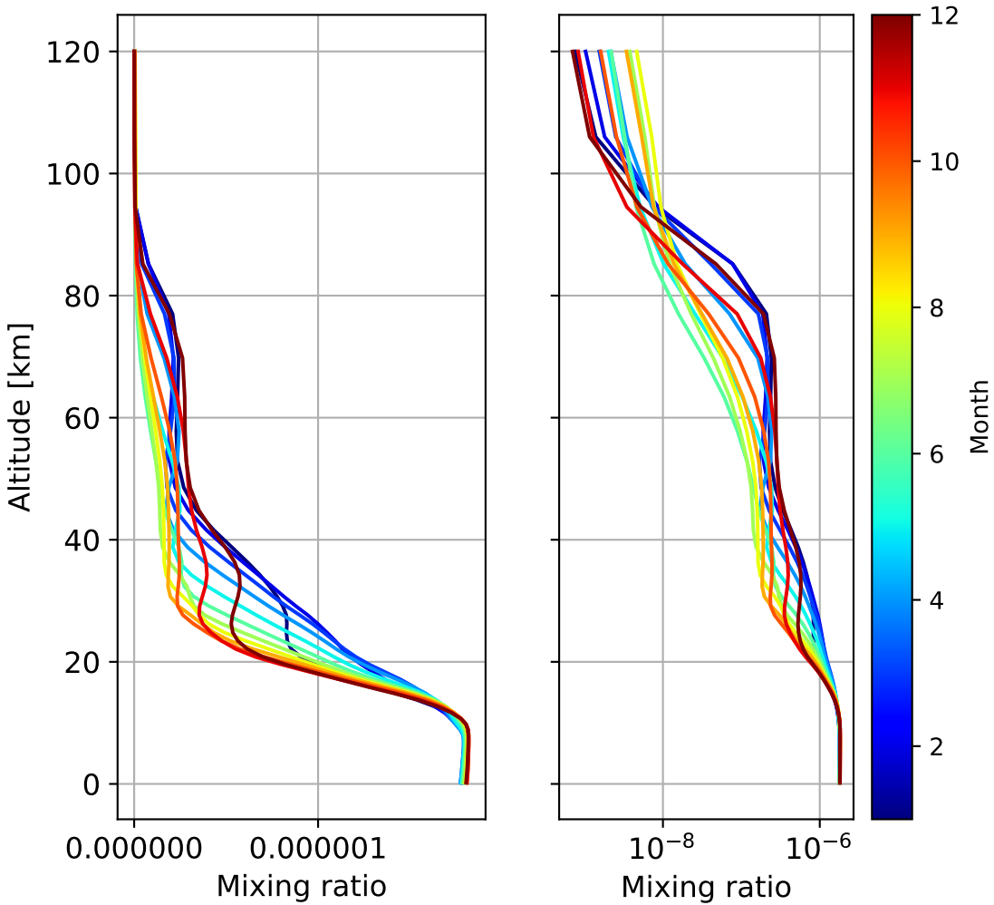
Monthly mean WACCM profile (interpolated to station grid) Arrival_Heights, -78.83N, 166.66E, 0.2kmasl
