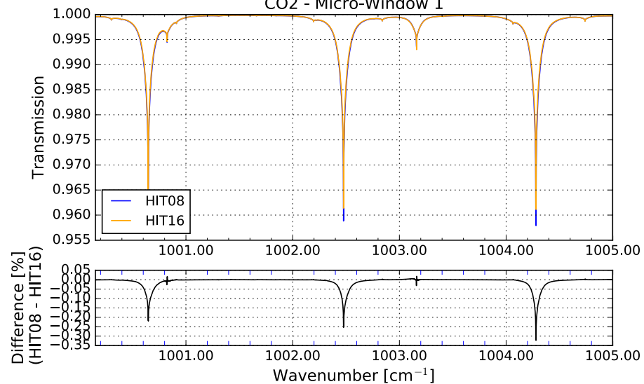
CO2 - Micro-Window 1
