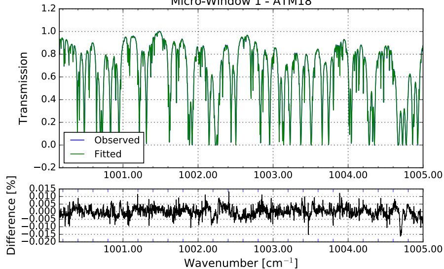
Micro-Window 1 - ATM18
