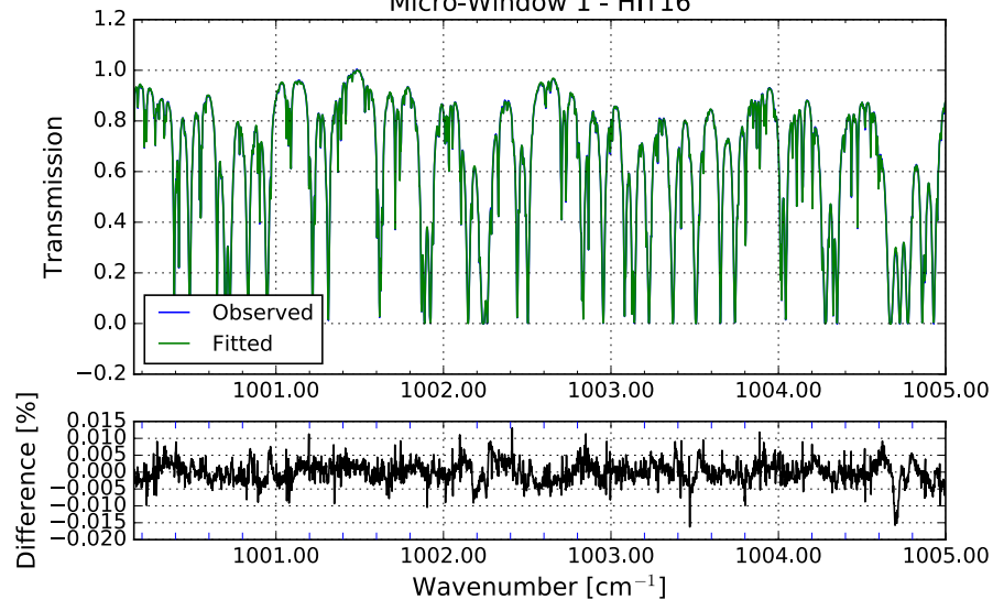
Micro-Window 1 - HIT16
