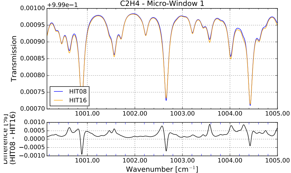
C2H4 - Micro-Window 1
