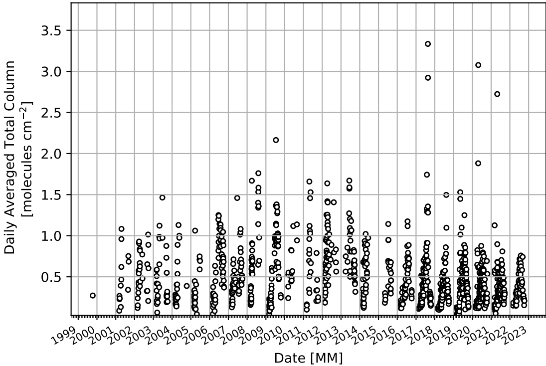
1e15 Time Series of Daily Averaged Total Column
