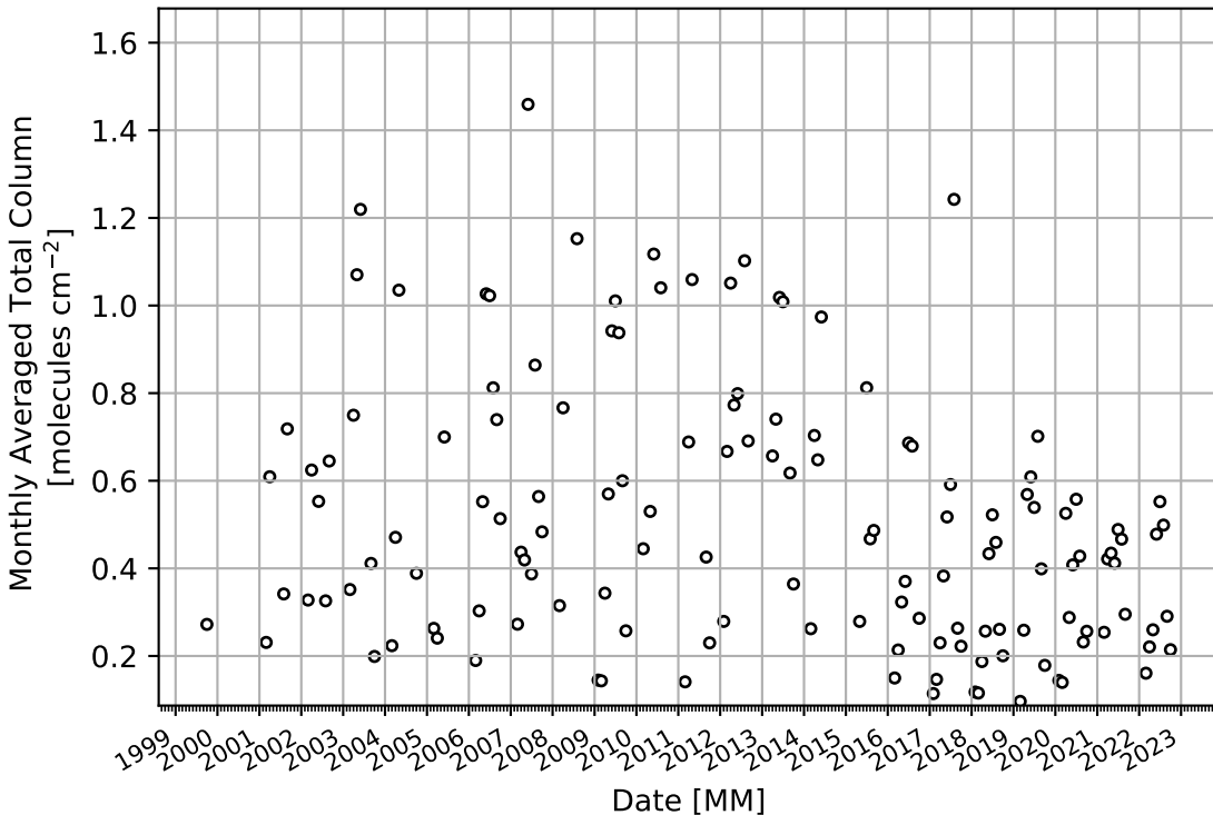
1e15 Time Series of Monthly Averaged Total Column
