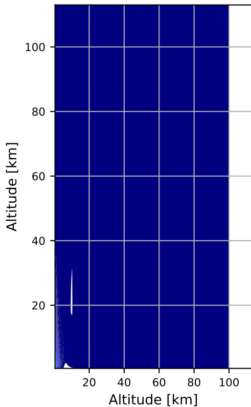
Averaging Kernel Matrix (Scale Factor)
