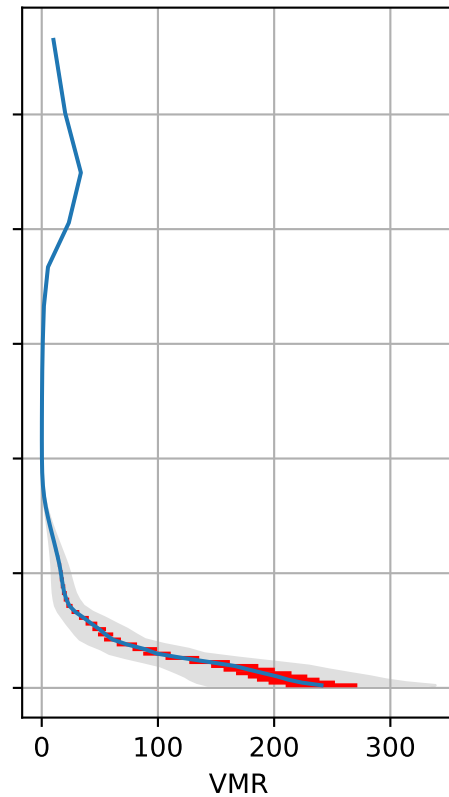
Systematic Error
