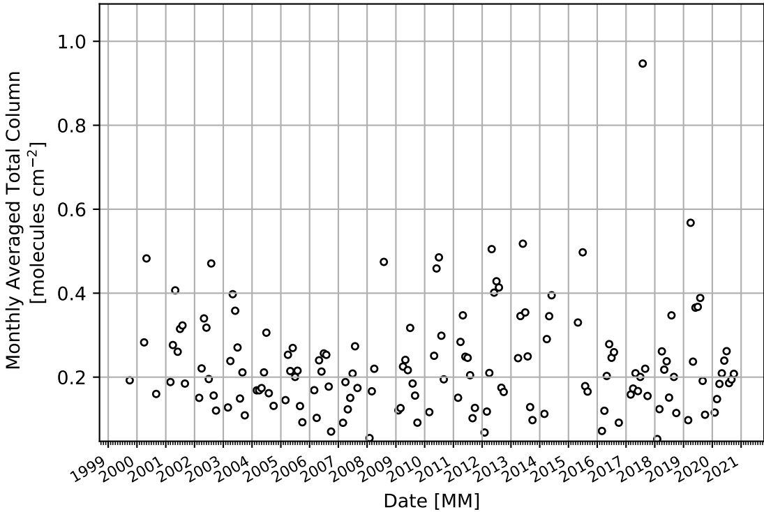
1e16 Time Series of Monthly Averaged Total Column
