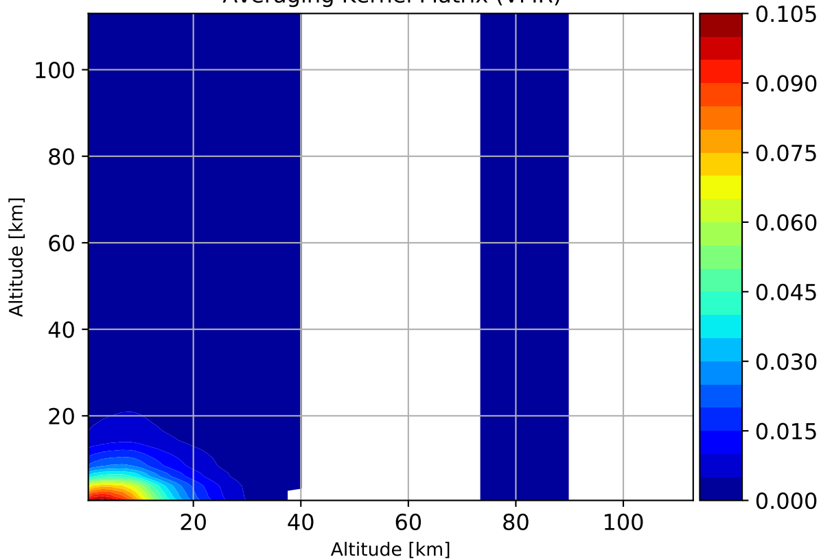
Averaging Kernel Matrix (VMR)
