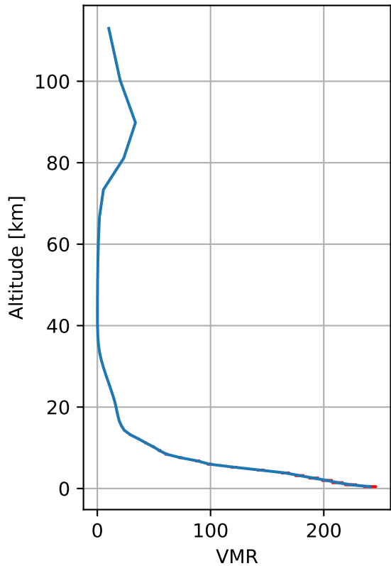
Random Error
