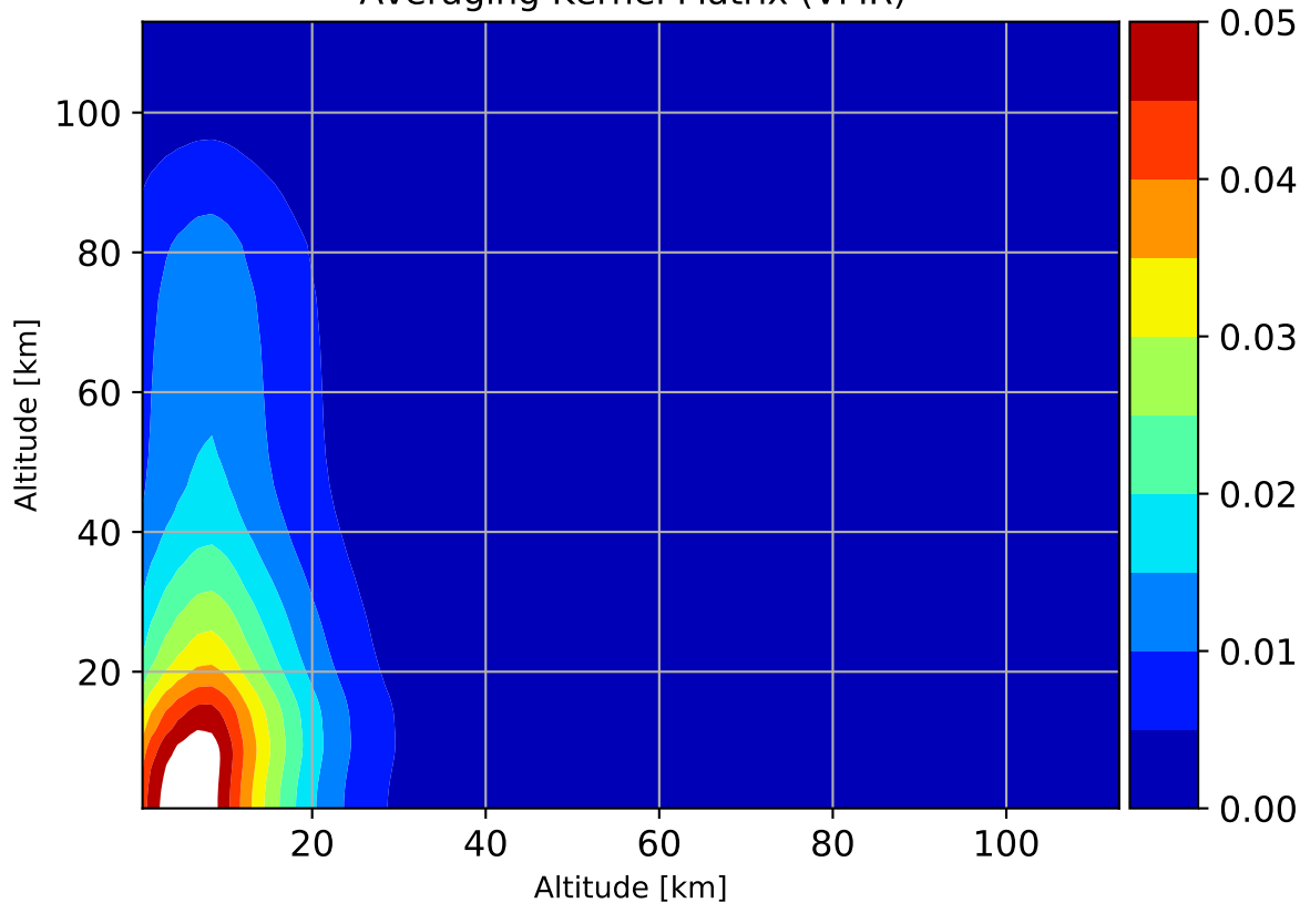
Averaging Kernel Matrix (VMR)
